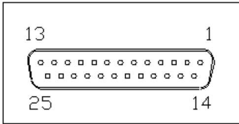
<D-SUB 25 Female Serial>
